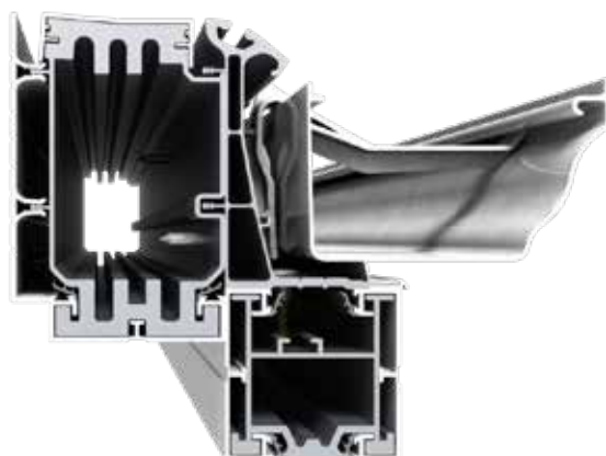
Combined Bolstered Eaves
