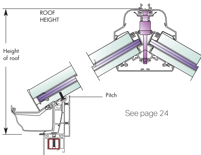
Diagram B - Slimline Ridge
