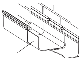
Jointing Sleeve
