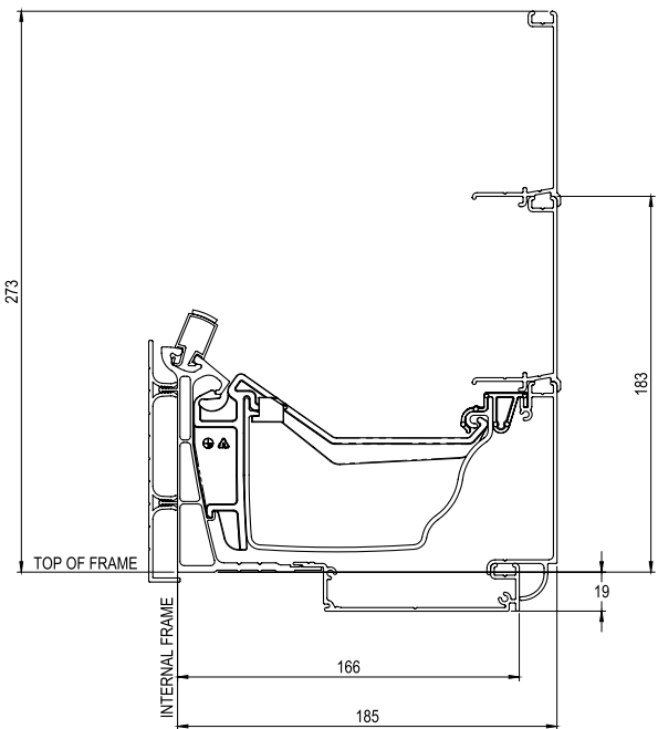
Flat fronted cornice
