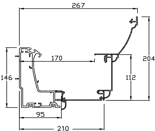
Super Duty Eaves Beam
