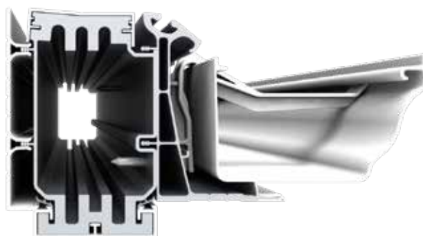
Eaves Super Bolster
