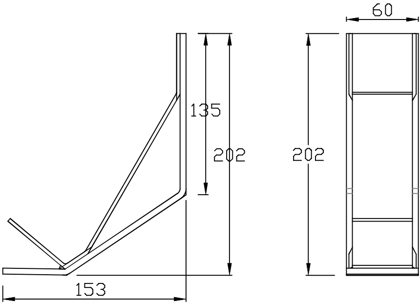
165 Hanging Bracket
