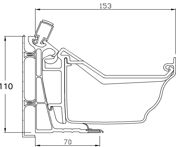
Standard Eaves Beam
