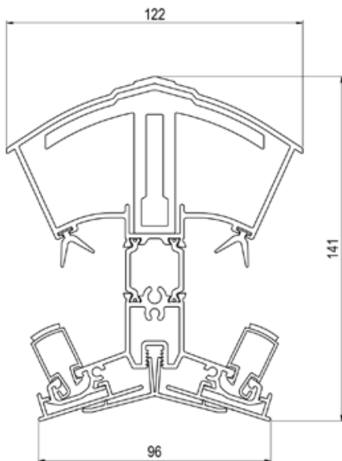
Slimline Ridge
