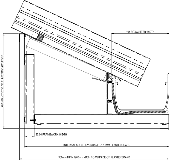
Box gutter below fascia
