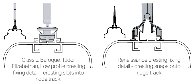
Pikestaff Finial, Renaissance Cresting
